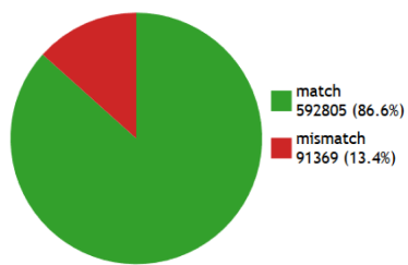
A Universal primers 16S rRNA-qPCR region coverage
