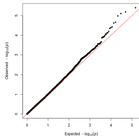
Q-Q plot of P values in LifeLines-DEEP cohort
