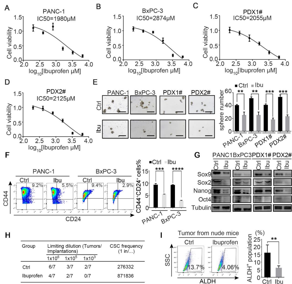
Supplementary figure 16. Ibuprofen suppresses cellular stemness in PDAC. (A-D) IC50 of ibuprofen in PANC-1 and BxPC-3 cell lines and PDX1# PDX2# primary cell lines were detected by CCK-8. 1mM ibuprofen was used in following experiments. (E) Adherent PDAC cell lines were pre-treated with 1mM ibuprofen for 48 hours (DMSO was used as control); and then cells were collected and cultured with serum-free medium for the following sphere formation assays. Ibuprofen abbreviated as Ibu in following experiments. Representative images were shown (left) and statistical analysis were shown (right). (F) Percentage of CD44 + CD24 + population were detected in indicated cell lines treated with 1mM ibuprofen by flow cytometry. Representative dot plots were shown (left) and statistical analysis were presented (right). (G) Western blot for stemness markers (Sox9, Sox2, Nanog and Oct4) were performed on indicated cell lines treated with 1mM ibuprofen. (H) In vivo limited dilution assay was performed to determine the effects of ibuprofen on CSC self-renewal of PANC-1 cells. Tumor incidence and CSCs probabilities were shown. (I) Percentage of ALDH + cells in harvested tumor tissues from panel H. PI was used to exclude dead cells and CD45 was used to exclude leukocytes and DEAB was used as negative control. Representative dot plots were shown (left) and statistical analysis were shown (right). Paired Student's t-test was used for statistical analysis of in vitro experiments
