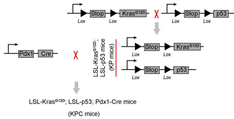
Supplementary figure 18. The breeding strategies for KPC mice models.
