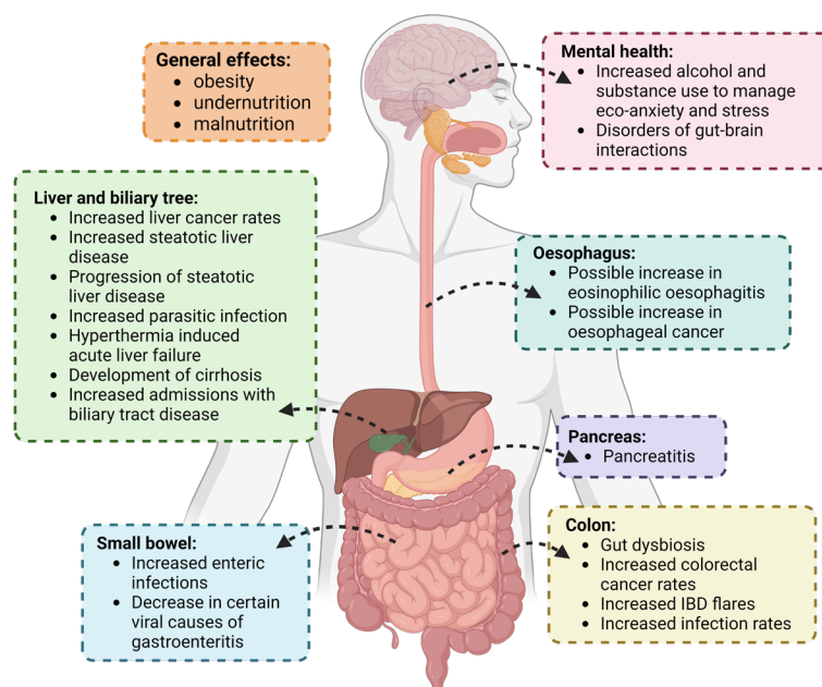
Figure 1 The effects of climate change on digestive health. IBD, inflammatory bowel disease.
