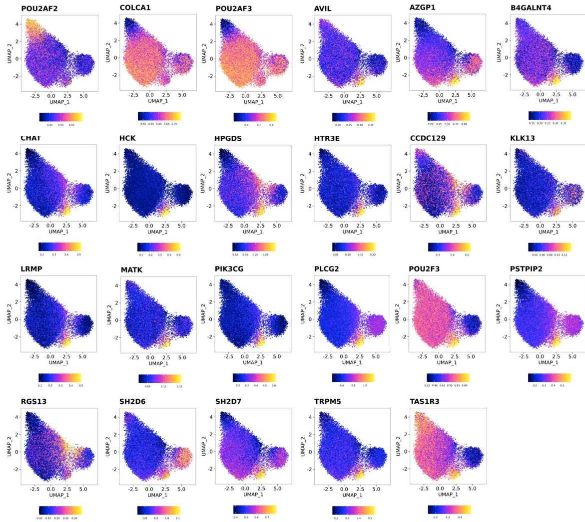
Figure S5. Chromatin at 11q23.1 trans-eQTL targets is exclusively accessible in tuft cells. Normalised accessibility of 11q23.1 cis- and refined trans-eQTL targets across individual cells.
