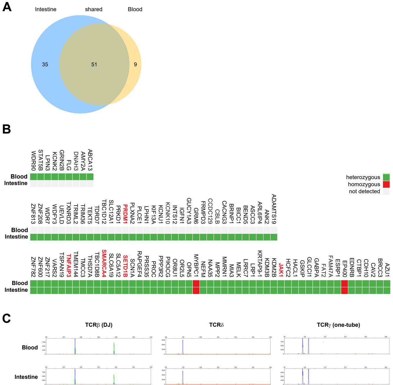
To Figure 1: Individual mutational profiles of RCDII cells derived from intestinal biopsy and freshly isolated from blood of P4. (A) Venn diagram illustrates overlapping and individual proportions of mutations detected in RCDII cells derived by culture from duodenal biopsies (Intestine) or directly sorted from peripheral blood (Blood) of the same patient (P4). (B) Heatmap details mutated genes detected in blood or intestinal-biopsy derived cells with gene names in red highlighting called potentially pathogenic variants as shown in Figure 1. (C) GeneScan electropherograms comparing TCR \beta (DJ), TCR \delta and TCR \gamma rearrangements in RCDII-cells freshly sorted from peripheral blood and cell-line derived from intestinal biopsy of P4.
