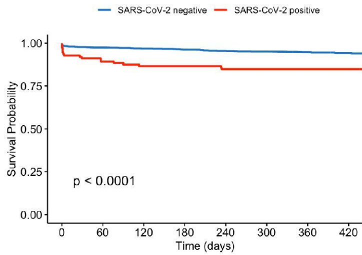
Figure S1: Kaplan-Meier survival curves of patients followed up after discharge from index admission for acute pancreatitis stratified by SARS-CoV-2 status
